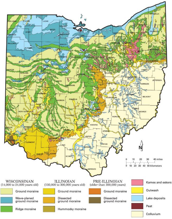
FIGURE 3. Glacial map of Ohio (Ohio Geological Survey, 2005). Approximately two-thirds of the state is covered by glacial materials.
