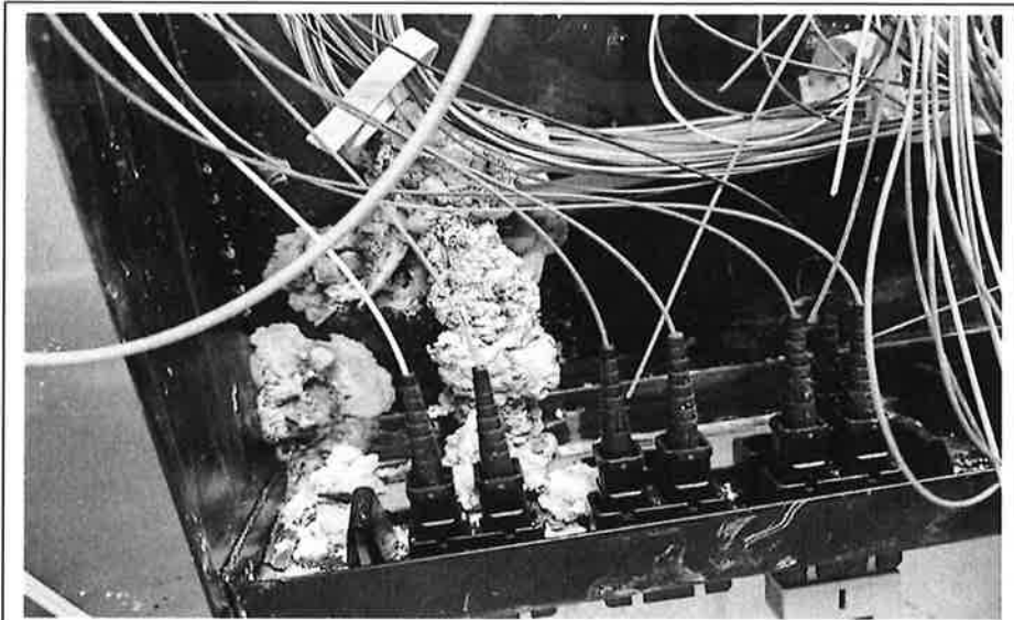
Figure 2.03-2 Crystalline Formations at End of Fiber-Optic Cables in Fiber-Patch Panels
